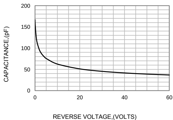
FIG.3-TYPICAL JUNCTION CAPACITANCE
